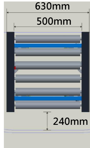
Figure 4: Roller Coaster (Unit: mm)
